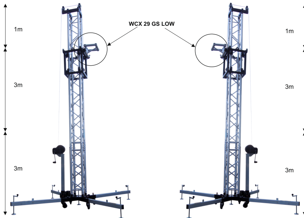
2x SET TORRE GS LOW (Torre elevadora Ground Support)
