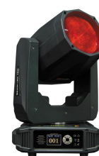
2 x BEAM LED 150 + RACK Móvil Beam 120W. 1 x LED BLANCO 80W. DMX Ch: 16/20. Apertura 0°-4°.
