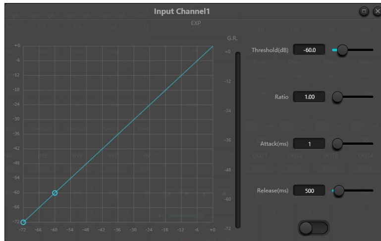
Fig.3.2 Expander
