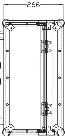
SECTION E-E
